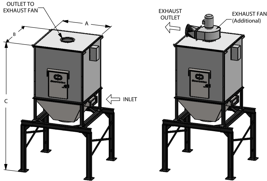
** ARRANGEMENT 1: (With top-mounted fan) ** Restrictions may apply
